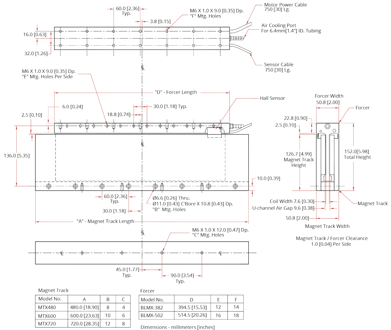
Figure 1-6: BLMX Model Dimensions
