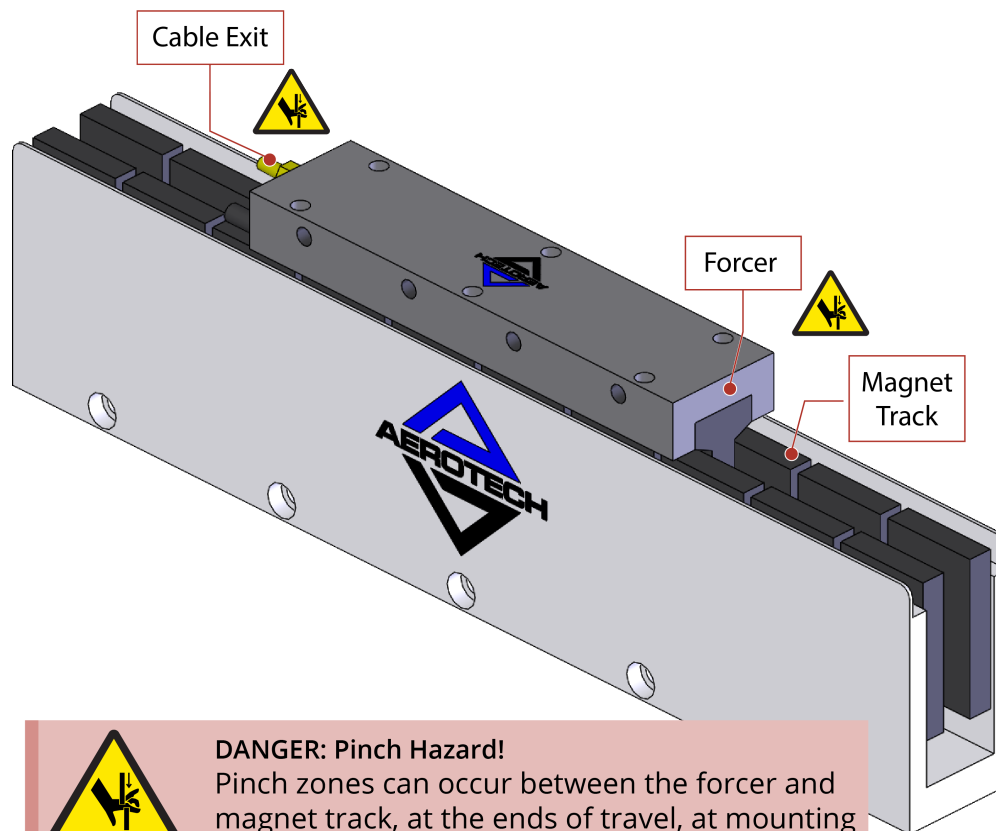
Figure 1: Typical Pinch Point Locations
