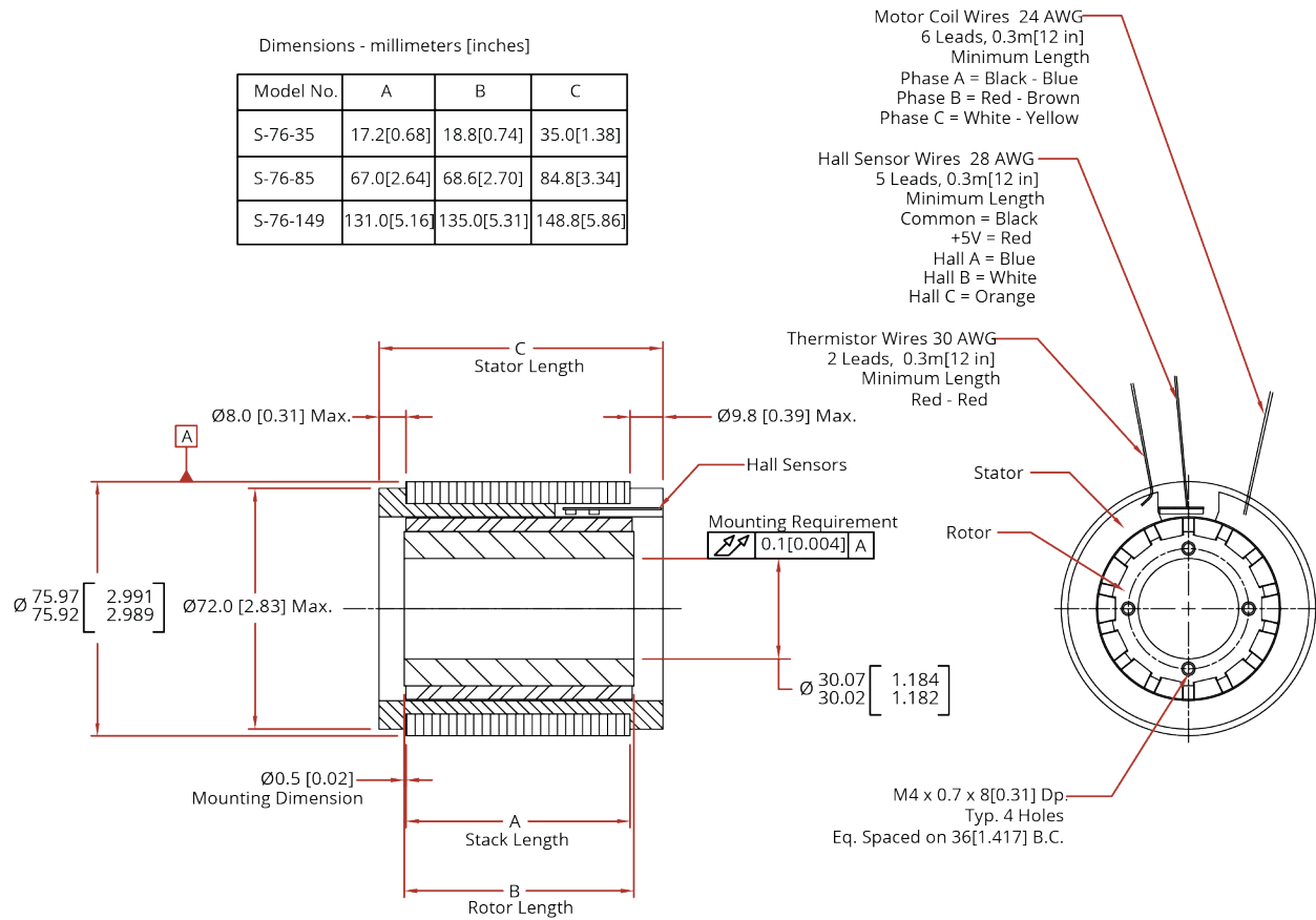
Figure 1-7: S-76 Dimensions
