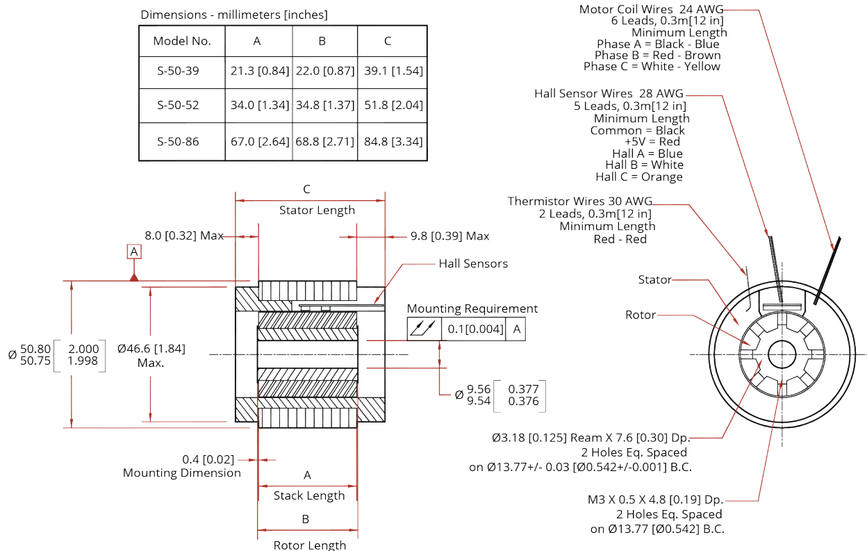
Figure 1-6: S-50 Dimensions
